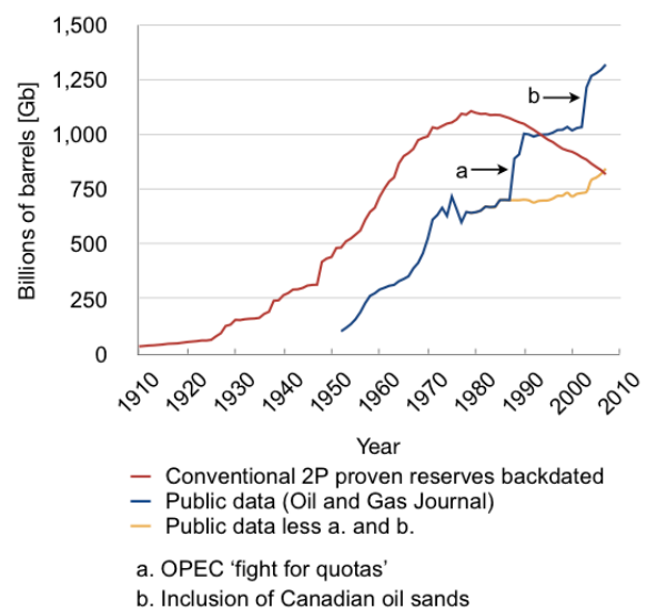
Figure 3: World cumulative crude oil reserves: backdated 2P data, OGJ data, and amended OGJ data. Sources: Constructed from data provided by Laherrère (2009b)
