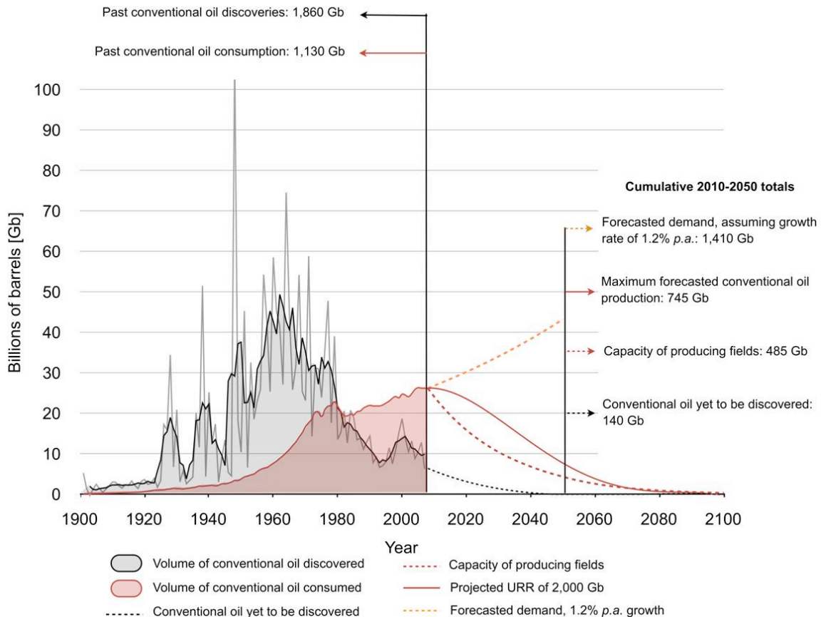
Figure 2: Annual backdated 2P conventional oil discovery, conventional oil consumption, and forecasted production and discovery. Sources: (Campbell and Laherrere, 1998; EIA, 2009a; IEA, 2008b; Laherrère, 2009b)
