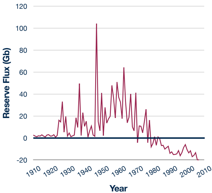
Figure 1: World 2P conventional oil reserve flux: additional volumes discovered less volumes consumed. Source: Data provided by Laherrère (2009b)
